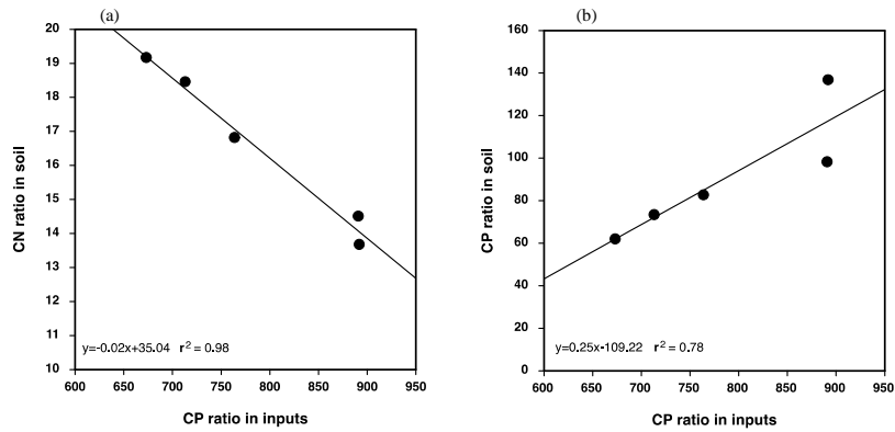
Figure 2. Relationships (a) between the C : P molar ratio in inputs and the soil C : N molar ratio and (b) between the C : P molar ratio in inputs and the soil C : P molar ratio in the Wagga Wagga field experiment.
