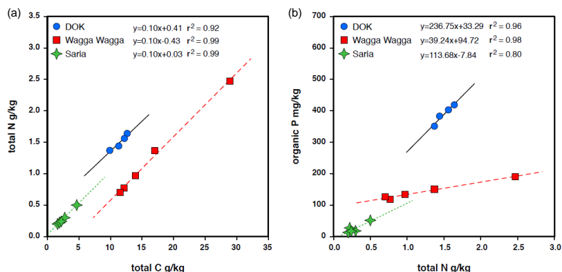
Figure 4. Relationships between soil C and soil N concentrations (a) and between soil N and soil organic P concentrations (b) in the three field experiment. Points in blue represent DOK, points in red represent Wagga Wagga, and points in green represent Saria. All relations are statistically significant at p < 0.05 .
